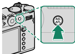
AEL/AFL 按钮 (AE/AF 锁)
