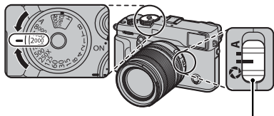
Diafragma-instelring
